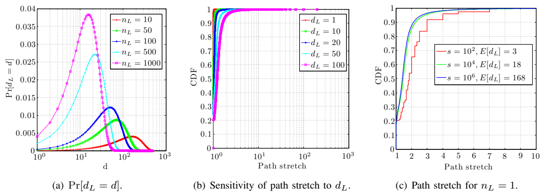
Fig. 7: Numerical analysis of path stretch ( s = 10^6 substrate networks).
