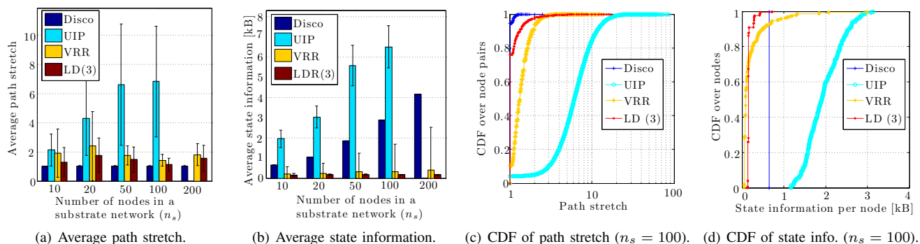
Fig. 8: Static multi-substrate network ( \alpha = 2.2 , \beta = 2.2 , s = 25 ).
