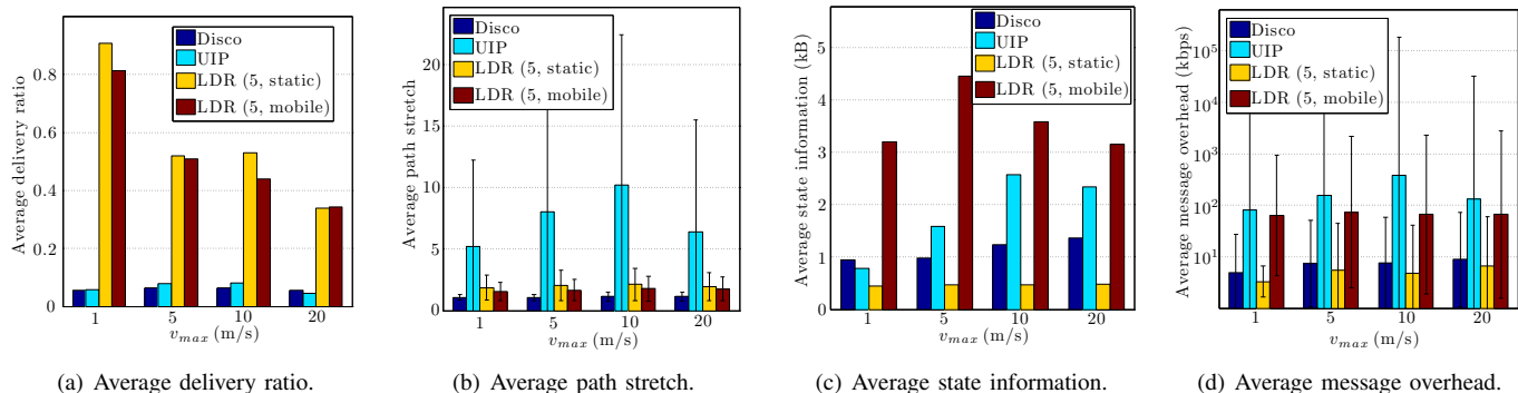
Fig. 9: Dynamic multi-substrate network.
