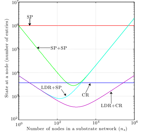
Fig. 6: State information (with intra-substrate routing) with n = 10^6 nodes.
